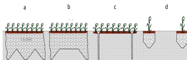
a - chisel processing; b - continuous processing with a strip recess; c - slotting; d - Strip-till
