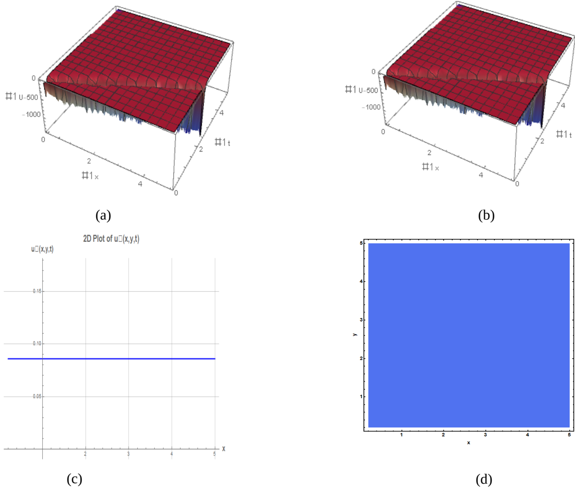
Figure 7: Wave profile for the solution obtained in eq (30) of u_7(x, y, t) with c = 1, k = 1, \alpha = \beta = \gamma = 0.5 and (a) 3D plot (b) 3D plot for \alpha = \beta = \gamma = 0.8 (c) 2D plot and (d) contour plot
