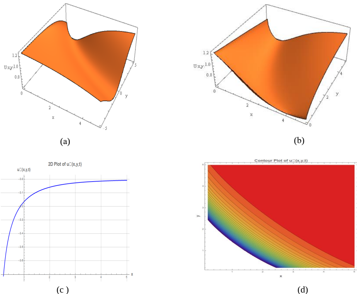
Figure 1: Wave profile for the solution obtained in eq (24) of u_1(x, y, t) with c = 1, k = 1, \alpha = \beta = \gamma = 0.5 and (a) 3D plot (b) 3D plot for \alpha = \beta = \gamma = 0.8 (c) 2D plot and (d) contour plot
