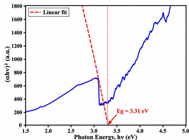
Figure 6: Direct-transition Tauc plot for the Synthesized \text{Co}_3\text{O}_4 Nanoparticles
