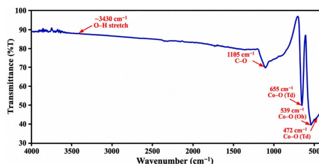
Figure 3: FTIR Spectrum of the Green-Synthesized \text{Co}_3\text{O}_4 Nanoparticles showing the Characteristic Low-wavenumber Metal–oxygen Bands
