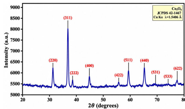
Figure 2: XRD Pattern of Green-Synthesized \text{Co}_3\text{O}_4 Nanoparticles
