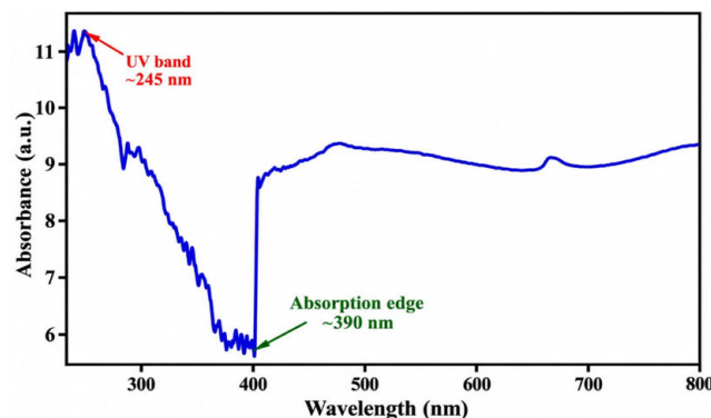
Figure 5: UV-Visible Absorption Spectrum of the Synthesized \text{Co}_3\text{O}_4 Nanoparticles
