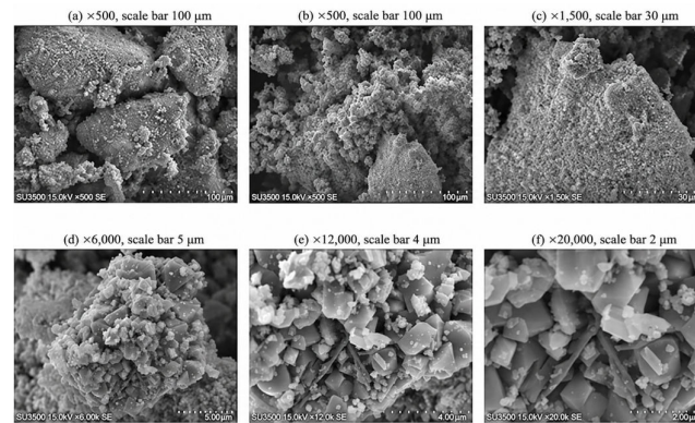
Figure 4: SEM Micrographs of Moringa oleifera -mediated \text{Co}_3\text{O}_4 at increasing Magnification
