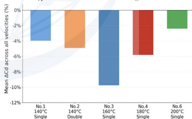
Figure 9: Mean \Delta Cd (%) Relative to No.5, Averaged Across All Flow Velocities (7–11 M/S), For Each Heat-Treated Specimen in the Airfoil-Type Model. No.3 (160°C Single-Side) Showed the Largest Overall Mean Reduction
