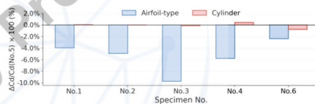
Figure 5: Relative Change in Drag Coefficient ( \Delta C_d , %) Of Heat-Treated Specimens Relative to The Untreated Fabric (No. 5). \Delta C_d Was Computed from Mean Cd Values Averaged Across All Flow Velocities (7–11 M/S)
