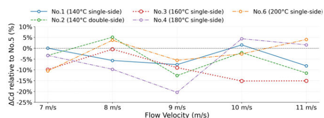
Figure 7: Velocity-Wise Relative Change in Drag Coefficient ( \Delta C_d , %) Compared to the Untreated Fabric (No.5) in the Airfoil-Type Model
