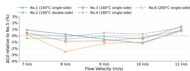
Figure 8: Velocity-Wise Relative Change in Drag Coefficient ( \Delta C_d , %) Compared to the Untreated Fabric (No.5) in the Cylinder Model
