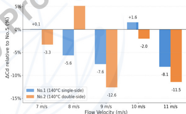
Figure 2: Comparison Of \Delta Cd (%) Between Single-Side (No.1) and Double-Side (No.2) Heat Treatment At 140°C In the Airfoil-Type Model. Negative Values Indicate Lower Cd Relative to No.5
