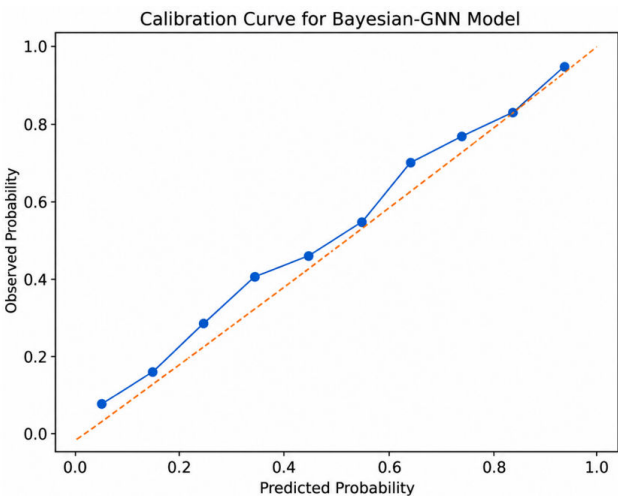
Figure 3: Calibration Curve for the Bayesian-GNN Framework
