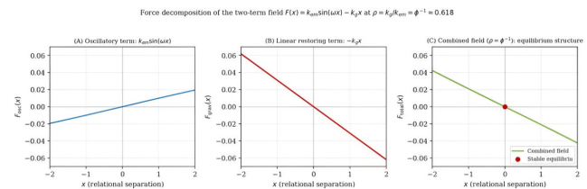
Figure 1: Decomposition of the deterministic field in one dimension. (A) Oscillatory term k_{em} \sin(\omega x) . (B) Linear restoring term -k_g x . (C) Superposition, with filled circles indicating the single stable equilibrium at x = 0 . Parameters: k_{em} = 0.05 , \rho = k_g/k_{em} = 0.618 , \omega = 0.2 .
