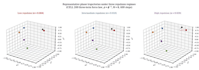
Figure 3: Representative phase trajectories for six particles under three values of repulsion strength \alpha , with \rho = \phi^{-1} = 0.618 fixed. Left ( \alpha = 0.004 ): attraction-dominated particles cluster toward the origin. Centre ( \alpha = 0.010 ): mixed regime trajectories spread but remain bounded. Right ( \alpha = 0.020 ): repulsion-dominated particles disperse, reaching the simulation boundary. Trajectories shown for 600 timesteps; final positions indicated by filled circles. Panels illustrate gradual qualitative differences, not sharp phase transitions.
